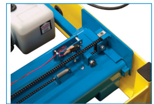
Linear motion structure with telescopic forks
